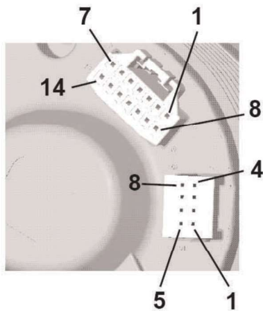
8 way connector Kit p/n A2C59510850
